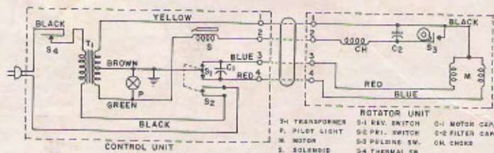
Fig. 4 — SCHEMATIC
