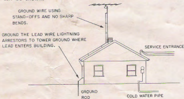
Fig. 3 — GROUNDING SYSTEM
